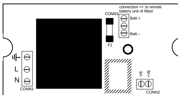
NC930 PCB LAYOUT
