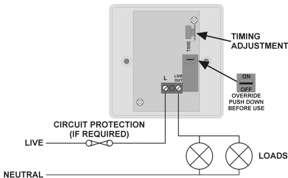
Diagram 1 Conventional wiring
