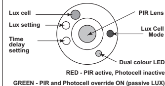
PIR head - key components
