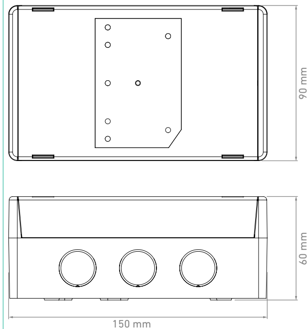
Figure 1: Intelligent Input/Output Unit dimensional drawing
