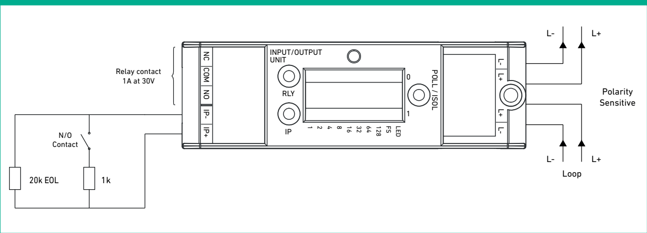
Figure 2: Intelligent Input/Output Unit standard resistive monitoring mode connectivity diagram
