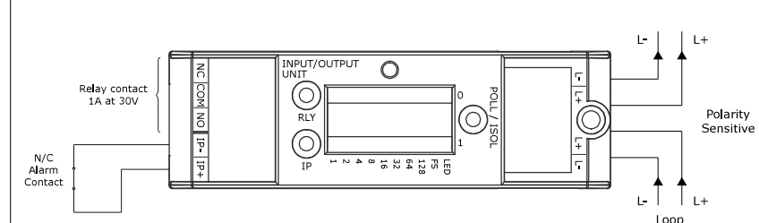
Fig. 3 Normally closed monitoring mode (Compatible with CoreProtocol only)
