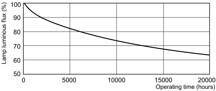
Lumen Maintenance Diagram - TL-D 15W/33-640 1SL/9
