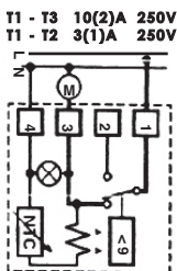
TH90C - With changeover contact (SPDT)
