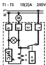
TH90 & TH90F - With normally closed contact (SPST)
