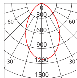
Photometric Diagram
