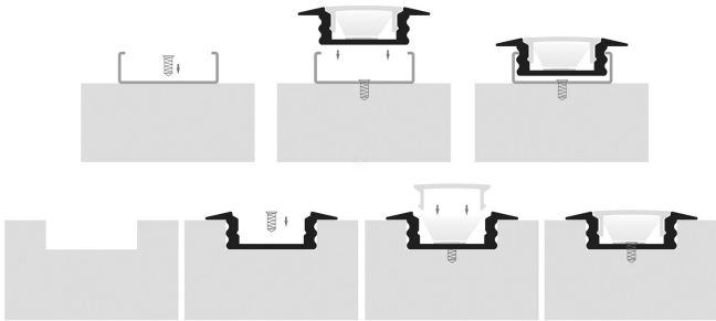
Sample Assembly Diagram
