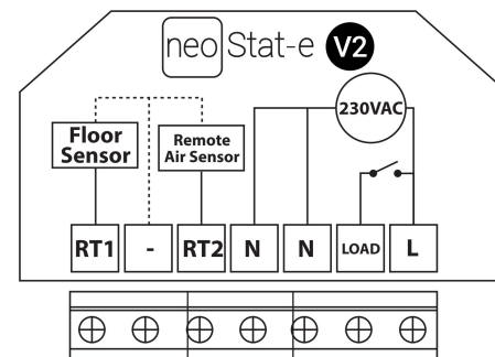
Wiring Detail
