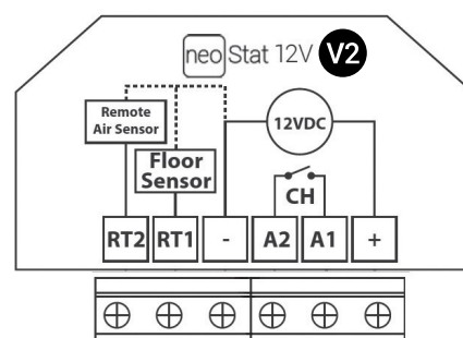
Wiring Detail
