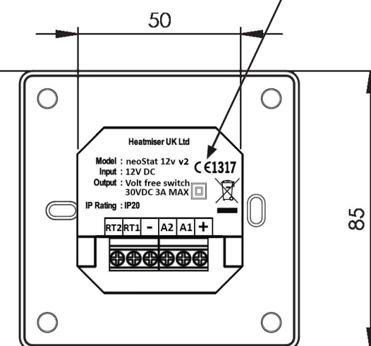
Wiring Detail
