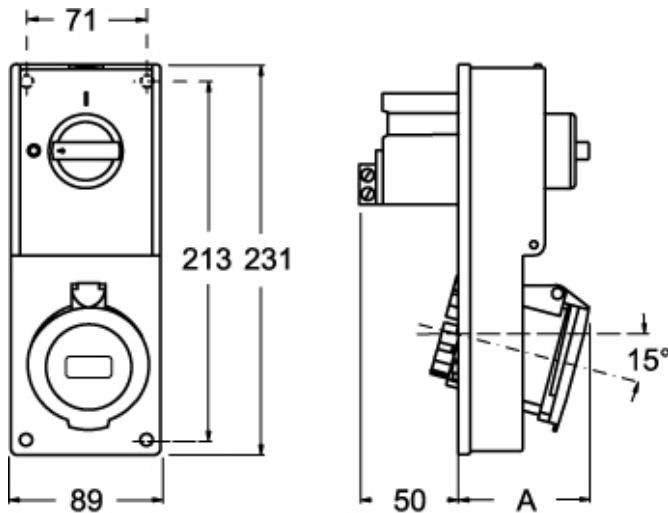
Catalogue drawings
