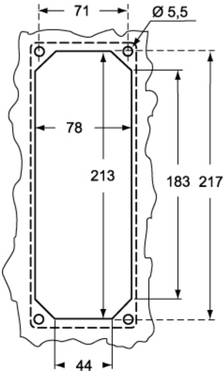
Catalogue drawings
