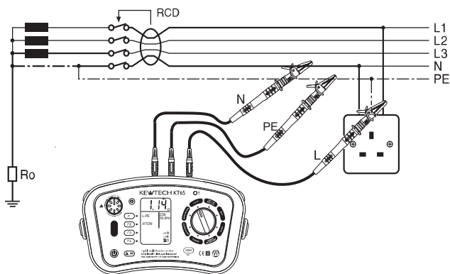
Fig.34 Connection for distribution
