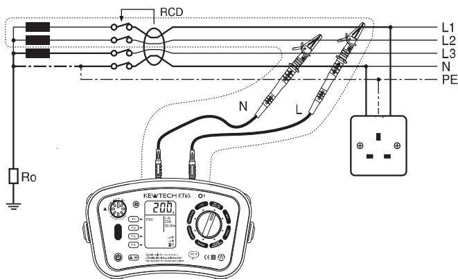
Fig.36 Connection for Line – Line measurement
