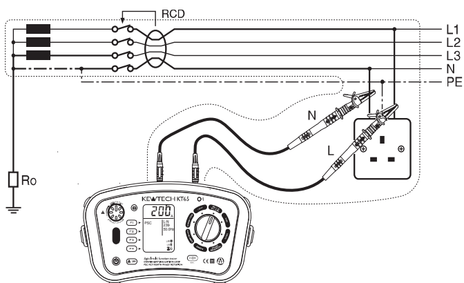
Fig.35 Connection for Line – Neutral measurement
