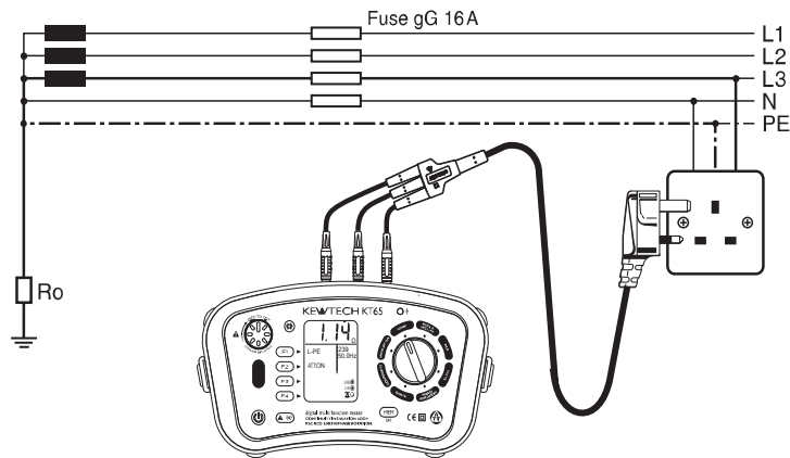
Fig. 33 Connection for using Outlet
