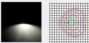
Asymmetric Forward Throw Optic 70°
