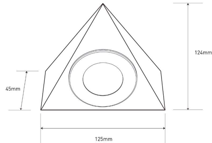
Dimension Diagram
