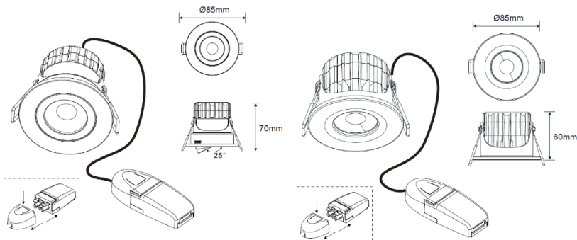
Dimension Diagram
