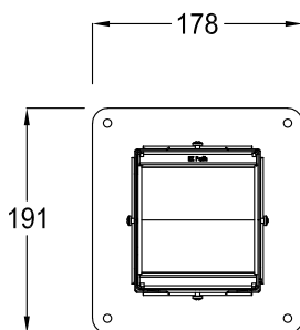
Opening size
