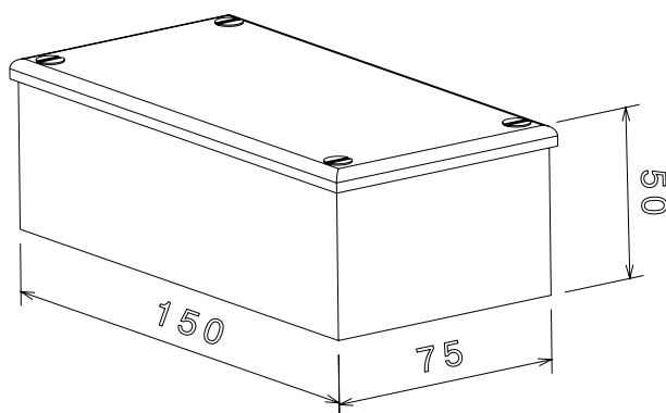
Isometric view
