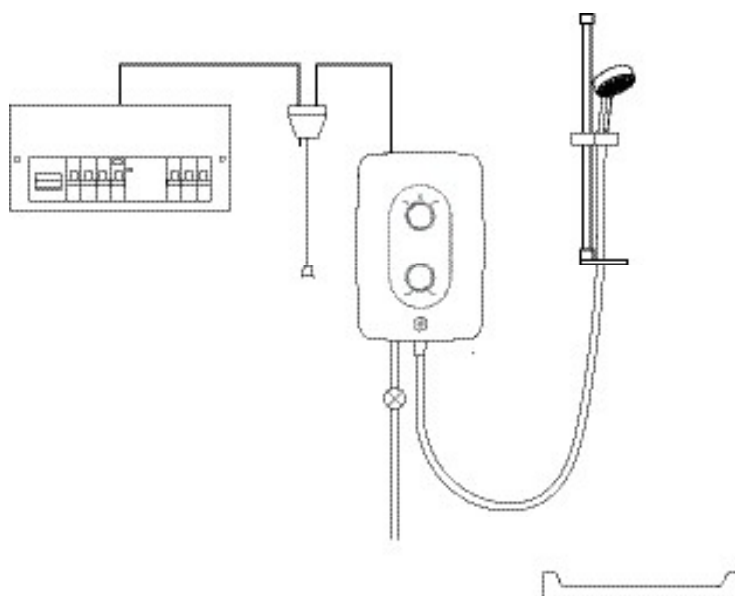
Plumbing and Electrical Schematic
