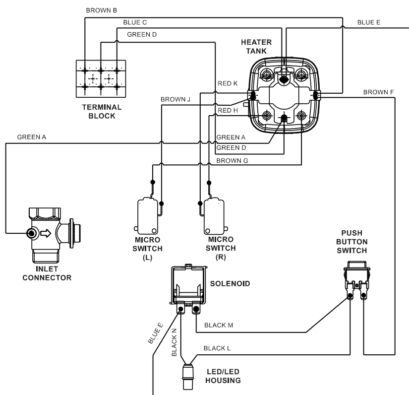
Internal Wiring Diagram
