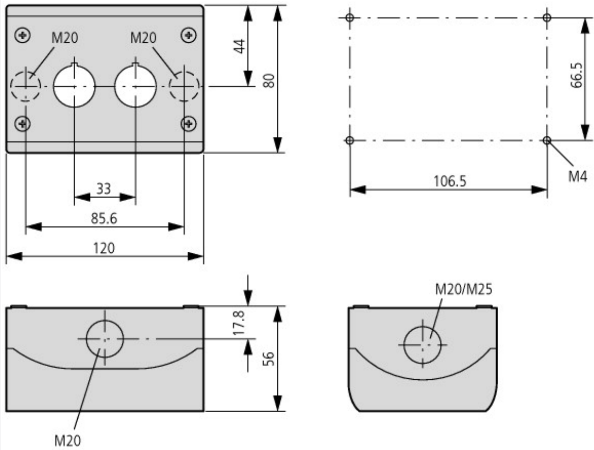
Premoulded cable entry: bottom 2 x M20, top: 1 x M20, side: 2 x M20/M25 (per side 1 x)
