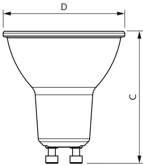
GU10 220-240V 4.9-50W 360lm 36D 2700K D
