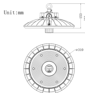
200W_Sensor
