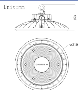
200W
