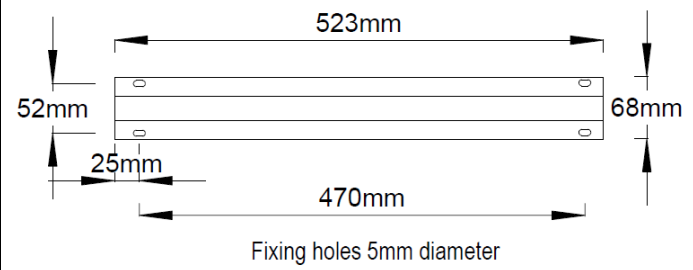
Mounting bracket fixing holes
