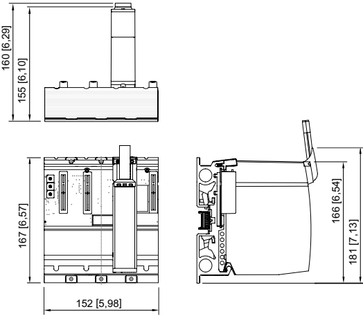
Power Modules 9445/32, 9445/35 + base 9496 (4 slots)
