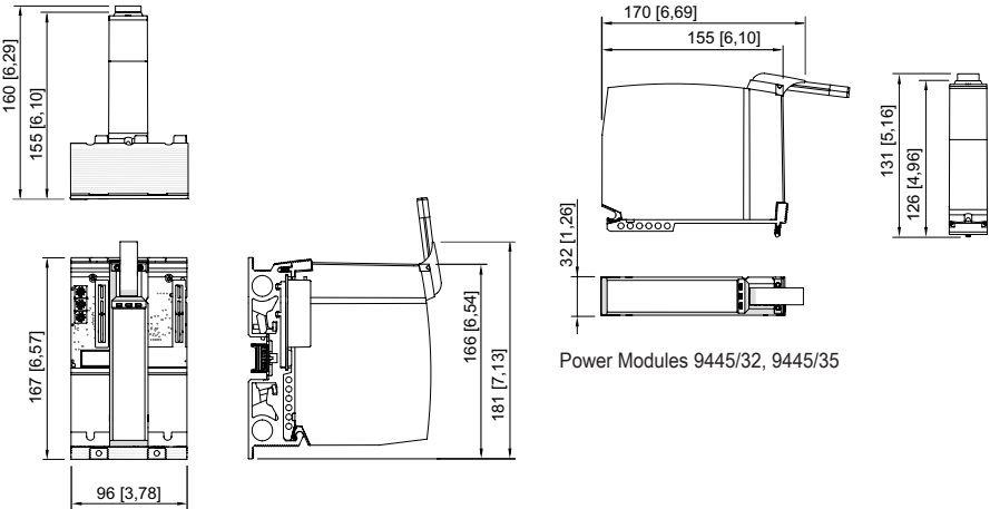
Power Modules 9445/32, 9445/35 + base 9496 (3 slots)
