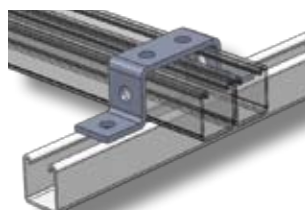
Size mm Cat. No. 2 HOLE 80mm STEP UP BRACKET TB173
