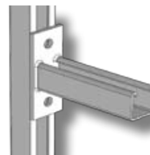
Size mm Cat. No. Size mm Cat. No. 150mm LONG ARM TC103-15 600mm LONG ARM TC103-60 300mm LONG ARM TC103-30 750mm LONG ARM TC103-75 450mm LONG ARM TC103-45
