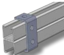
Size mm Cat. No. 3 HOLE 20mm TOP HAT TB174
