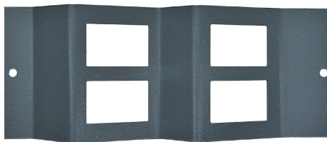
ST0302/W 4 Way Data Wave Plate 4 x 37x22mm LJ6C Module Cutouts
