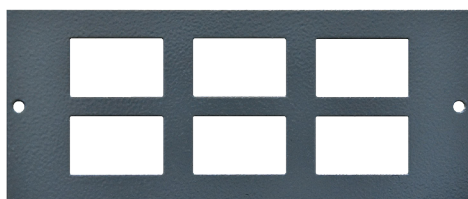
ST0306 6 Way Data Plate 6 x 37x22mm LJ6C Module Cutouts
