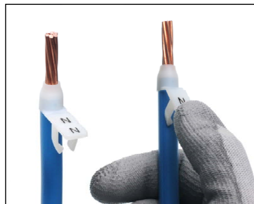
Push the safety collar over the cable and fold down the tag to clip into place.
