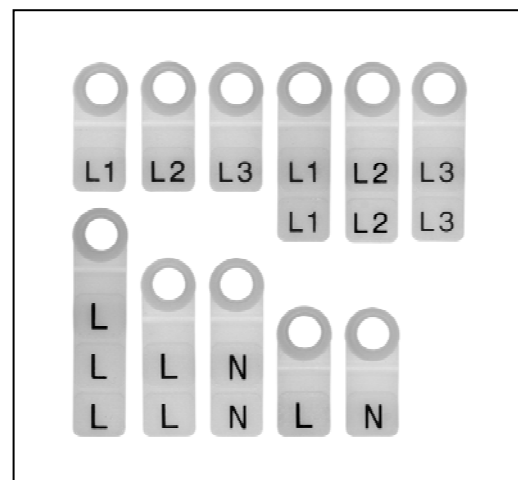
Push the safety collar over the cable and fold down the tag to clip into place.
