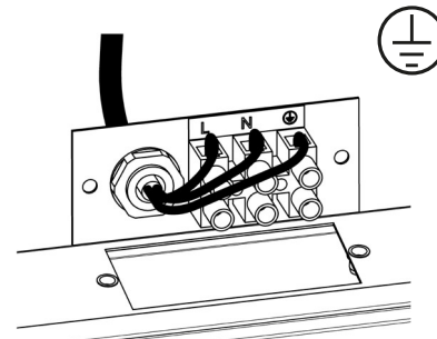
Figure 4: Electrical Connection
