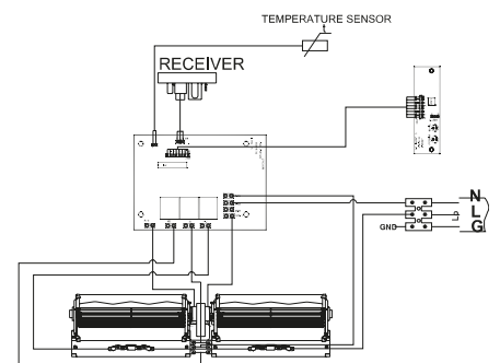
Figure 5: Electrical Wiring
