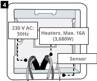
Install a 50 mm deep electrical back box (35 mm min.) in your preferred thermostat location. Pull wires (heater, supply and sensor(s) through back box and complete terminal wiring.
