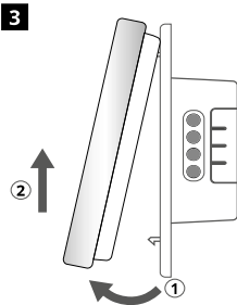
Release the display as shown.
